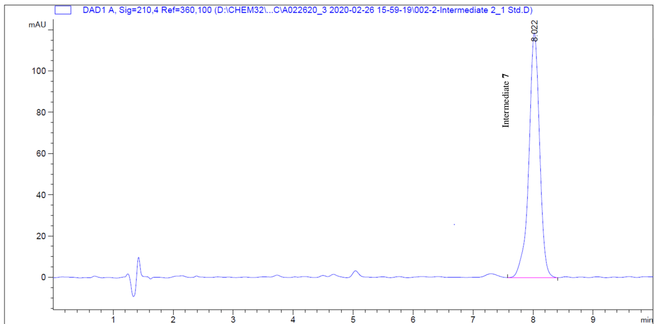
Figure 5. HPLC-DAD Chromatogram for Intermediate 7 standard
