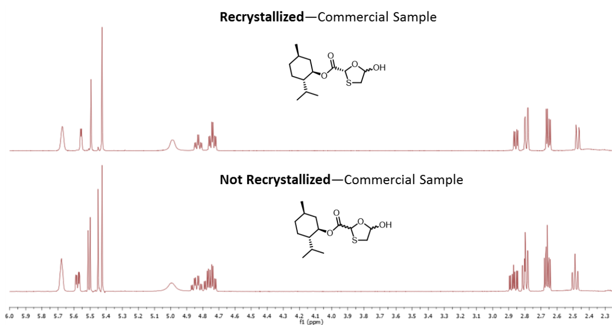
Figure 16: Recrystallization of commercial 1 demonstrating removal of two diastereomers. ^1\text{H} NMR taken in toluene- d_8 .
