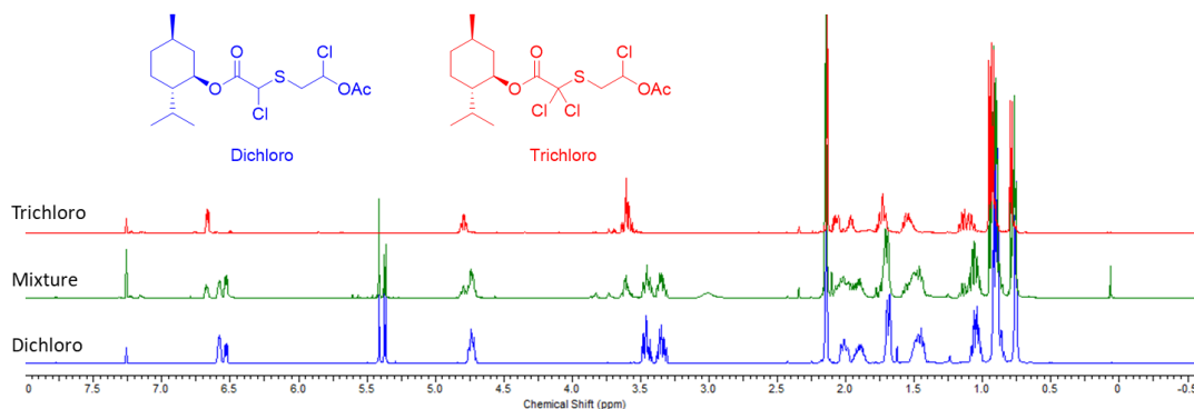
Figure 11: Trichloro compound formation with excess of sulfuryl chloride
