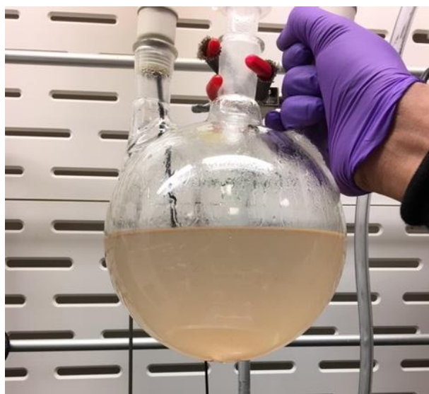
Figure 13: Dispersion of dichloroacetate in acetonitrile/water solvent system.
