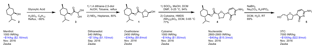
Figure 1: Current manufacturing route for lamivudine.
