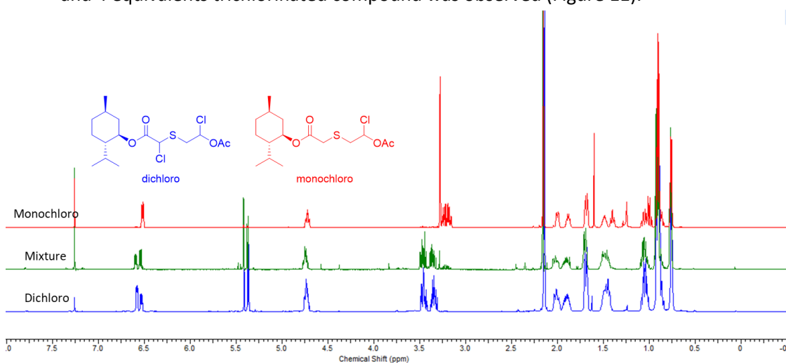
Figure 10: Monochloro compound formation at 2.0 and 2.1 equiv of sulfuryl chloride
