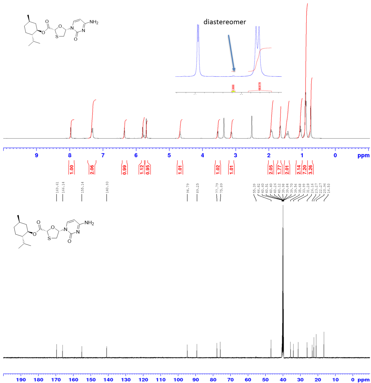
Figure 24: Coupling 1 with cytosine. 1 made from M4ALL process.
