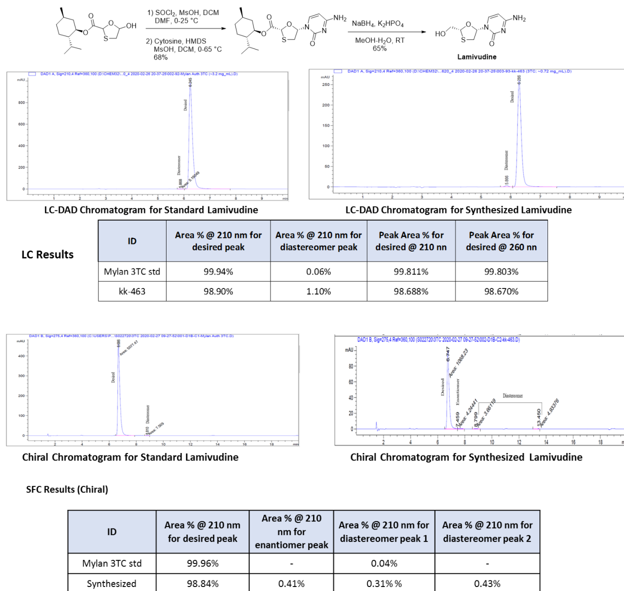
Figure 23: Production of lamivudine from 1. 1 made from M4ALL process and matches authentic material.
